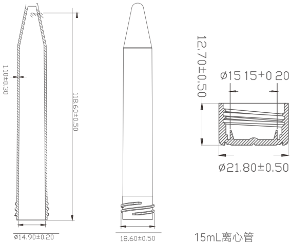
15mL离心管
